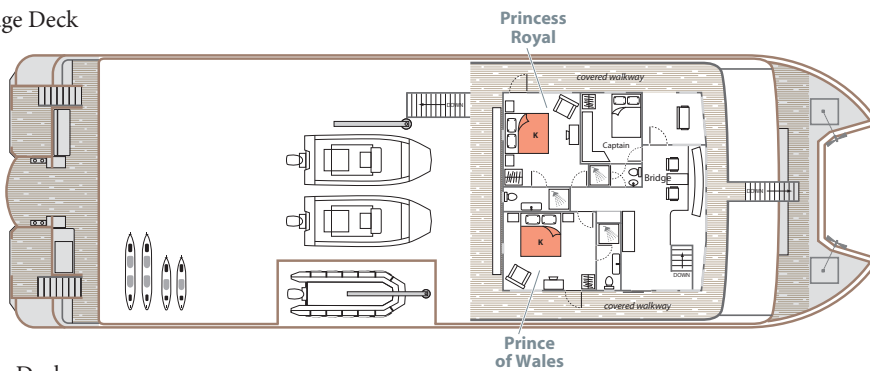
Main Deck
